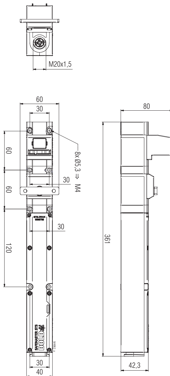
YRXK01M/K Clearance tolerances \pm 2\%
