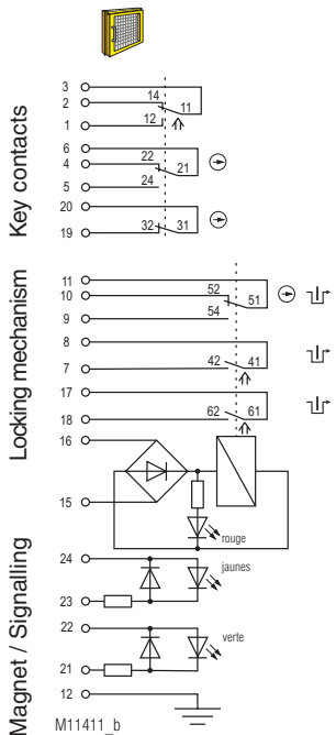
Fig. 2: Solenoid locking deactivated: Magnet released, 1st key removed 2nd Key inserted
