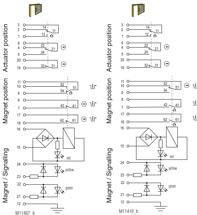
Fig. 3: Blocking function deactivated: Magnet locked, actuator removed and not pluggable Door open
